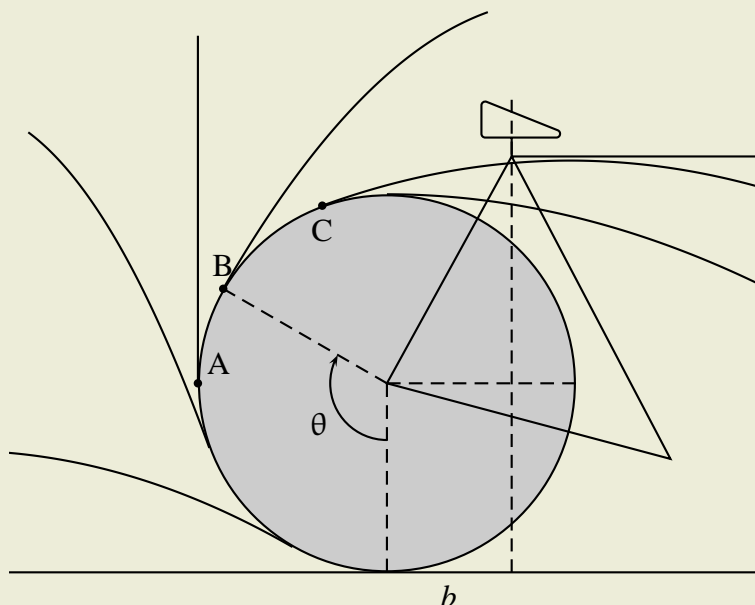
FIG. 3 – trajectoires relatives
